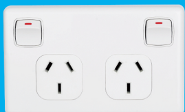
LBL008N/DP Double Switched Socket 10A (double poles) 250V Dimension/packing 118×73mm 10×10pcs
