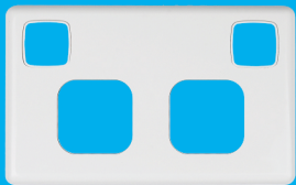
LBL008N/P Double Switched Socket Plate Dimension/packing 118×73mm 20×10pcs
