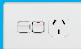
LBL016 Single Switched Socket 10A with Removable Extra Switch 15A 250V Dimension/packing 118×73mm 10×10pcs
